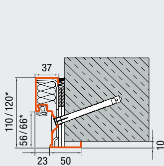
DryFix frame with diagonal fixing (Unplastered brickwork/concrete)
