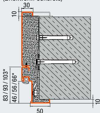
Corner and counter frame with concealed plug-and-screw fitting and counter frame with fitting by welding (Unplastered brickwork / concrete)
