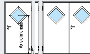
Diamond-shaped glazing
