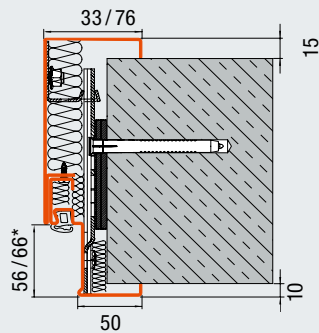
Double-shell profile frame with concealed plug-and-screw fitting and mineral wool backfill (Brickwork/unplastered brickwork / concrete, also for plastered brickwork)
