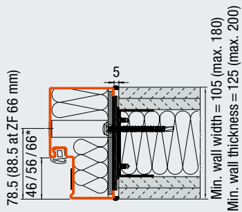
Block frame with flush-fitting cover caps as concealed plug-and-screw fitting in the opening (Partition wall)
