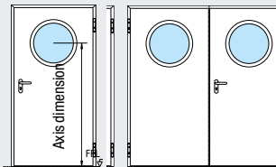
Round glazing
