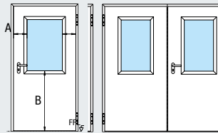
Glazing view 2
